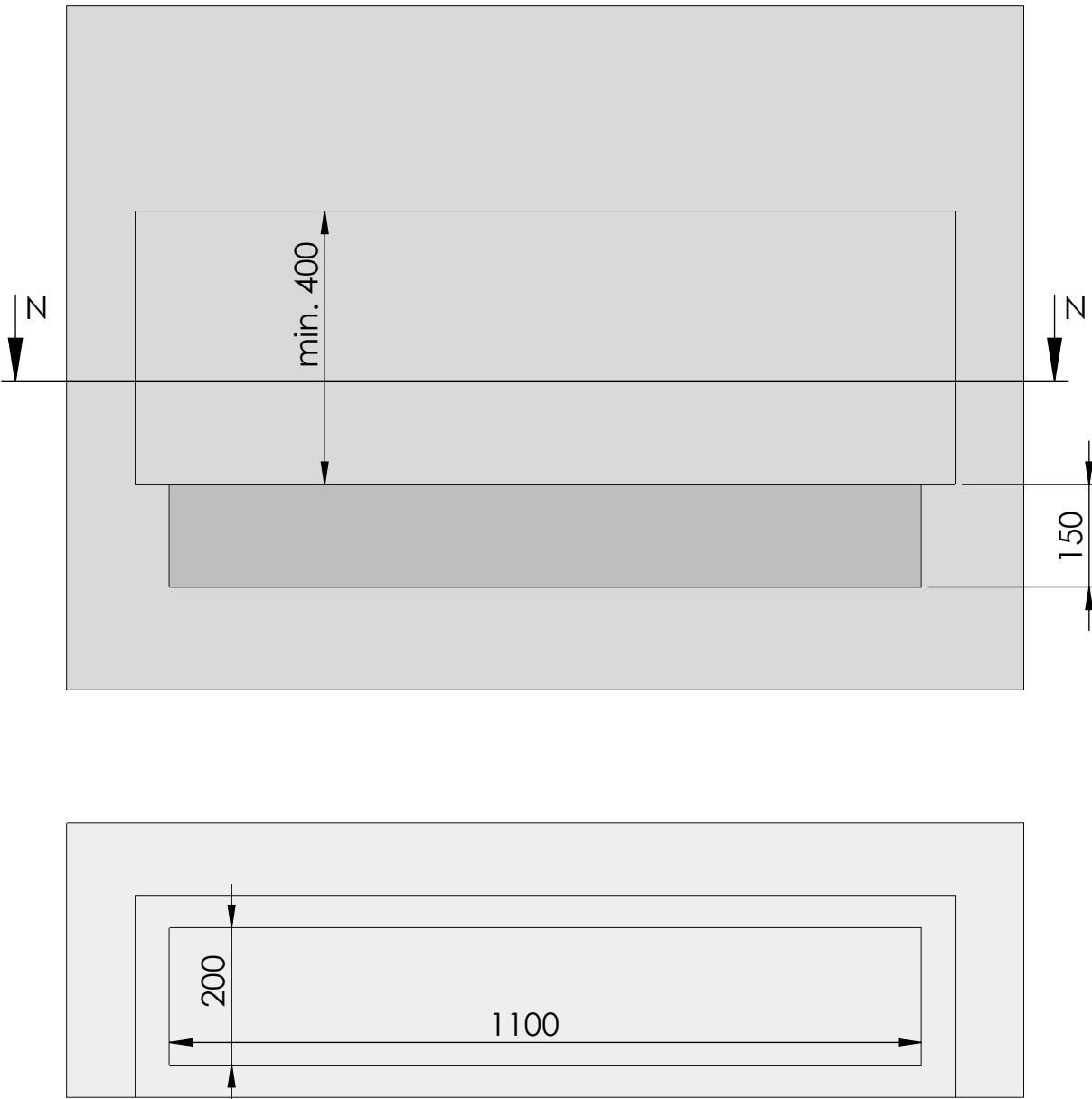
SECTION N-N
